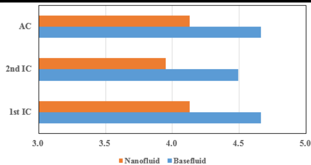
Fig. 8: Tube side Pr comparison
