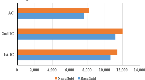
Fig. 4: Tube side heat transfer coefficient comparison
