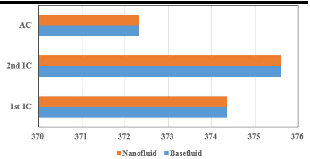
Fig. 5: Shell side heat transfer coefficient comparison
