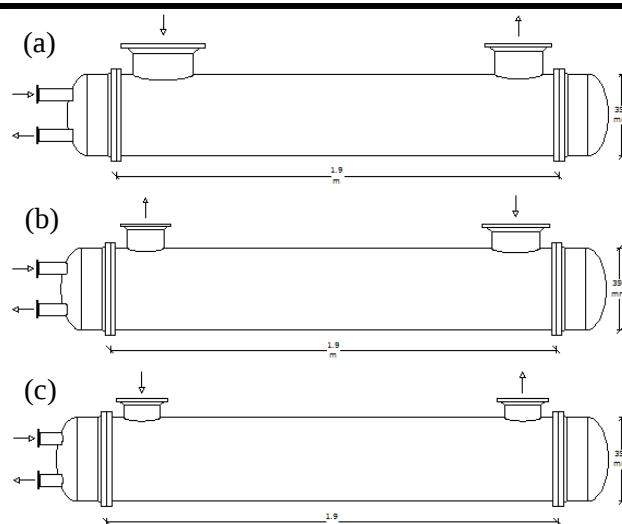
Fig.3: Sketch layout of 1 st intercooler (a), 2 nd intercooler (b), and aftercooler (c)
